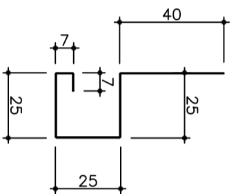
腰水切り C-250 2m (0.4t)
