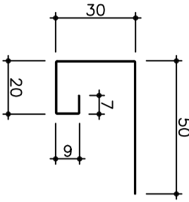
廻り縁 SK-101 2m (0.4t)
